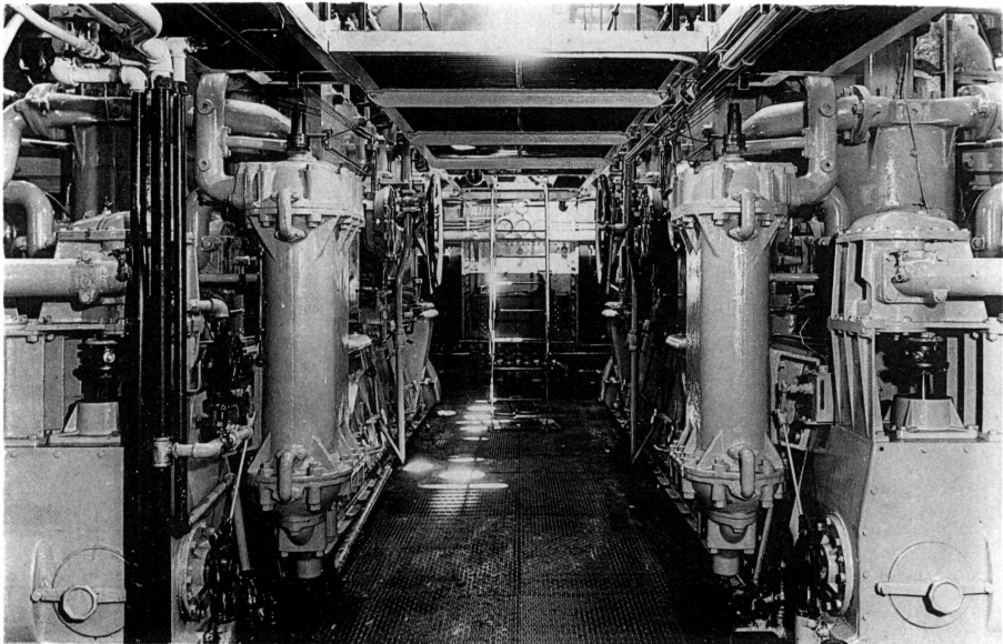
Figs. 21, 22 Engine room
