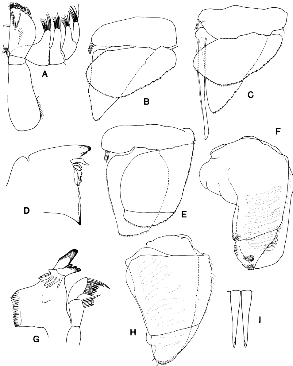
Figure 36. Paracilicaea stauros sp. nov. (A) Maxilliped; (B) pleopod 1; (C) male pleopod 2; (D) right mandible; (E) pleopod 3; (F) pleopod 5; (G) left mandible; (H) pleopod 4; (I) penes.
