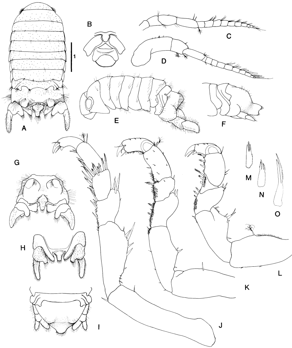
Figure 35. Paracilicsea stauros sp. nov. (A) Male, dorsal view; (B) frons; (C) antenna; (D) antennule; (E) male, lateral view; (F) female, pleon in lateral view; (G) male pleotelson, posterior view; (H) male pleotelson in ventral view; (I) female pleon in dorsal view; (J) pereopod 7; (K) pereopod 2; (L) pereopod 1; (M, N, O) carpal setae from pereopod 1, enlarged.
